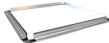
Mez Connector With Gasket and Fasteners
