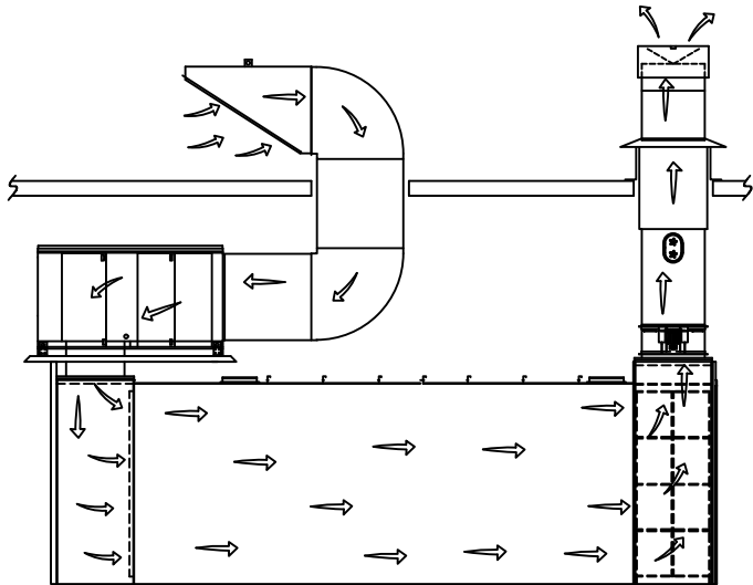
*BOOTH MOUNTED AMU (HORIZONTAL UNIT)
