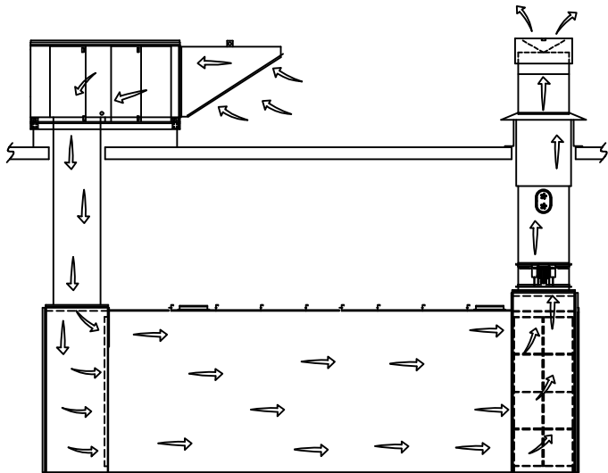
*ROOF MOUNTED AMU (HORIZONTAL UNIT)
