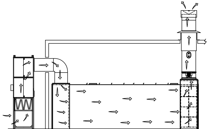
*VERTICAL OUTSIDE MOUNTED AMU
